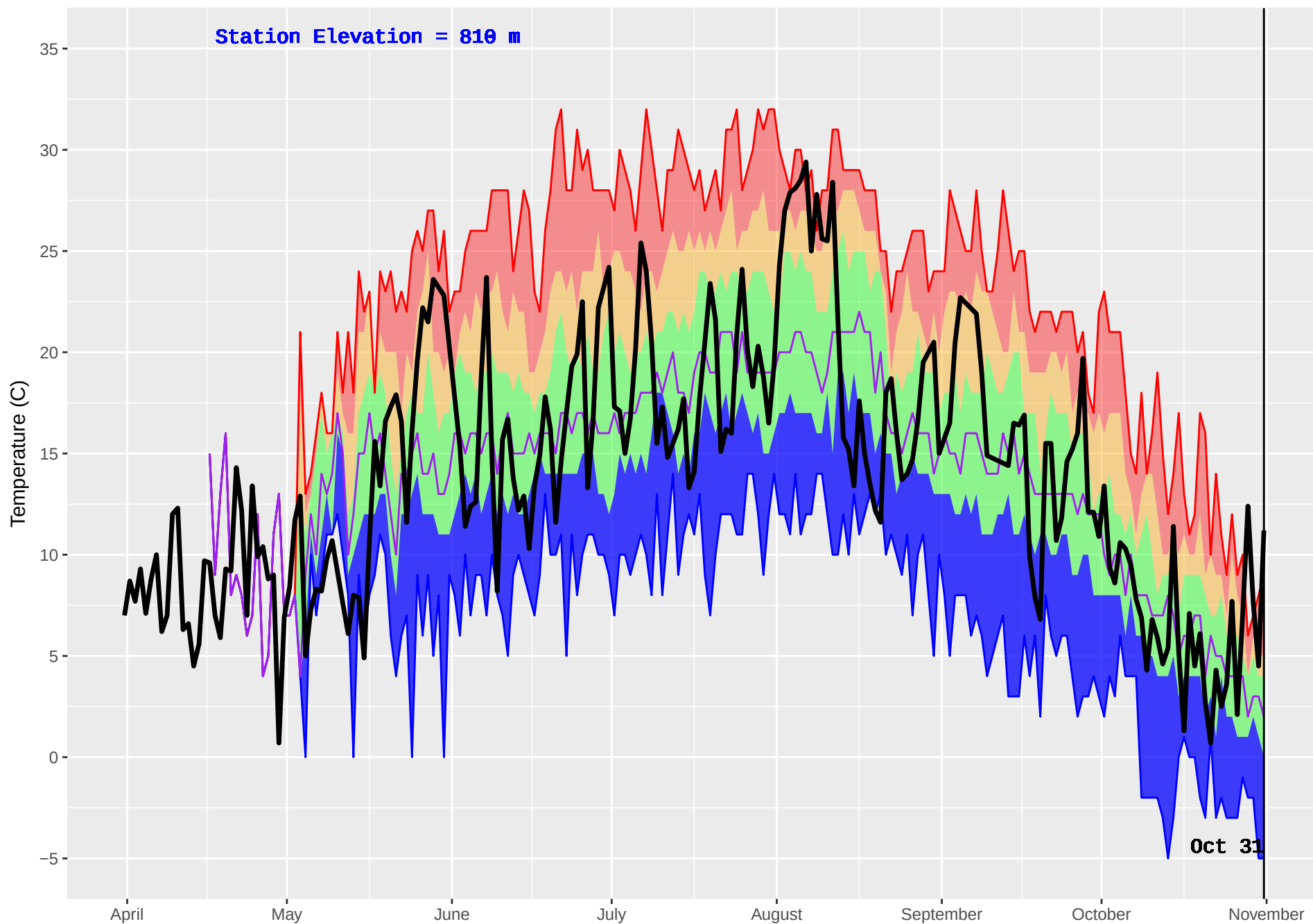
MCBRIDE LAKE (180) : Historical (1990–2016) and Current (2017) Noon Temperature
