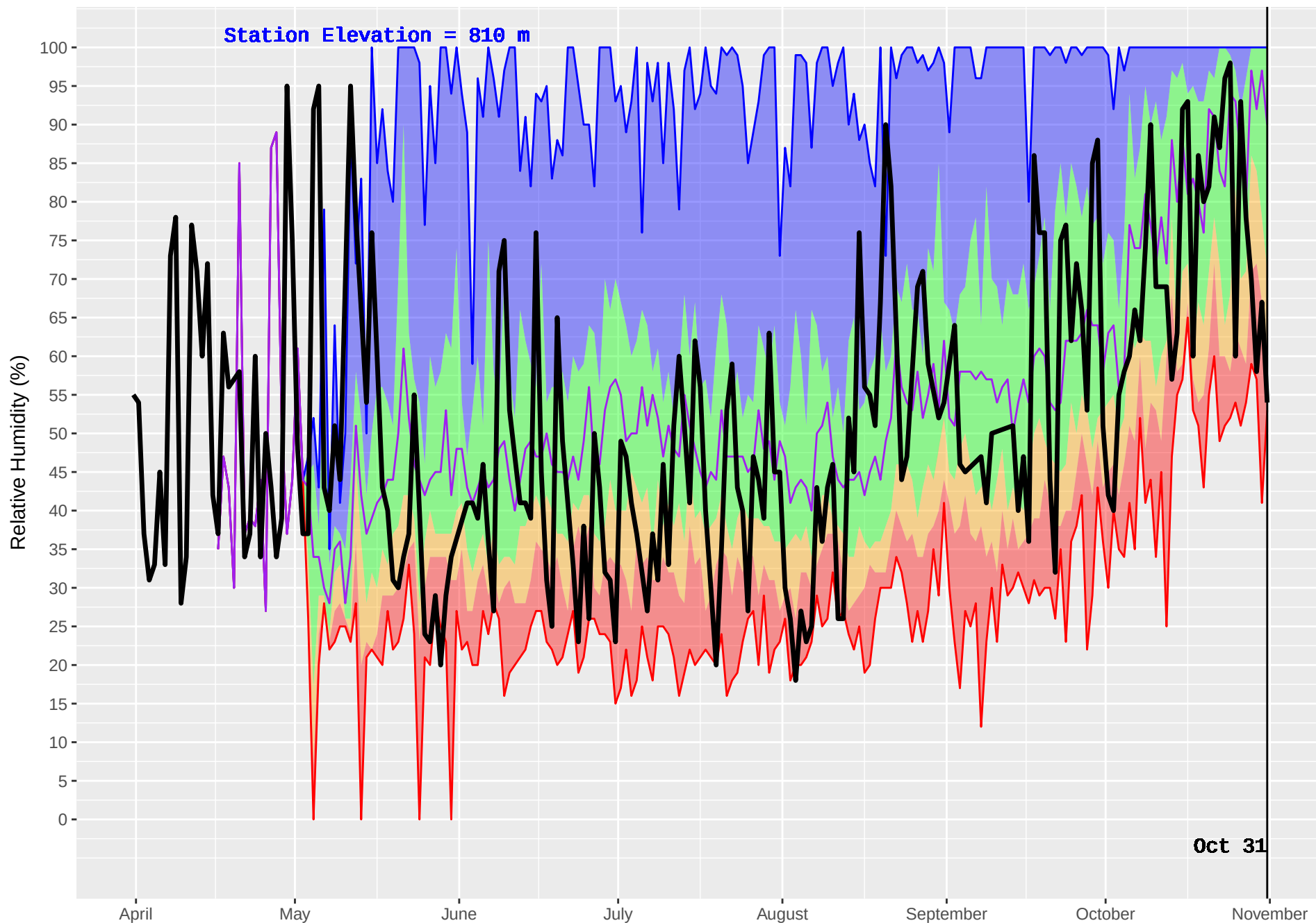
MCBRIDE LAKE (180) : Historical (1990–2016) and Current (2017) Noon Relative Humidity
