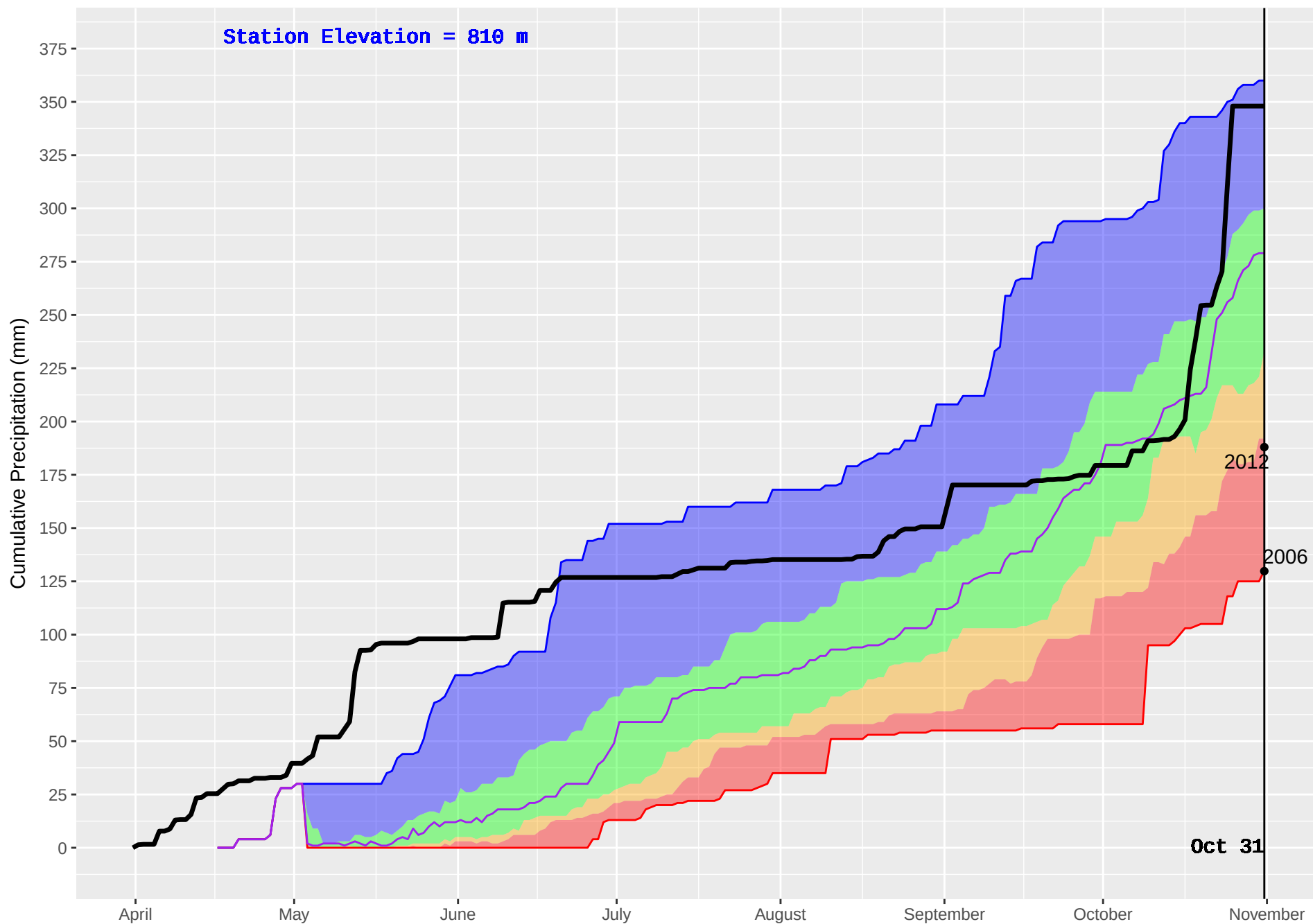
MCBRIDE LAKE (180) : Historical (1990–2016) and Current (2017) Noon Cumulative Precipitation
